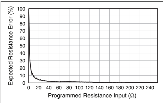
Figure 1. Expected resistance error between 0 and 255 \Omega
