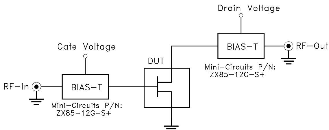
Fig 1. Block Diagram of Test Circuit used for characterization. (DUT soldered on Mini-Circuits Test Board TB-471+)
