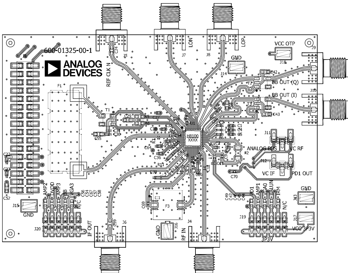
Figure 53. Evaluation PCB
