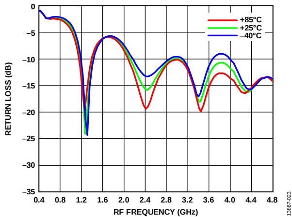
Figure 23. RF Return Loss vs. RF Frequency over Temperature (Optimize RF Return Loss by Adjusting Capacitor C12, see Figure 52)
