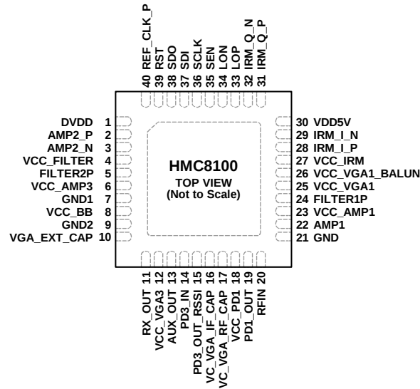
Figure 2. Pin Configuration
