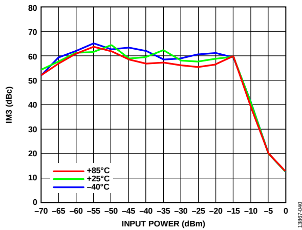
Figure 40. IM3 vs. Input Power over Temperature, RF = 1 GHz
