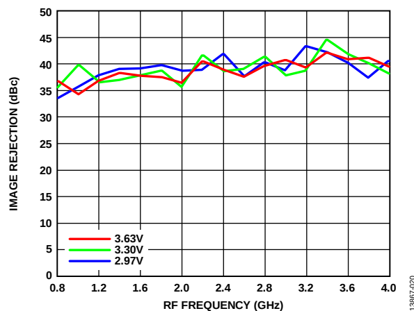
Figure 20. Image vs. RF Frequency at Various V_{CCQ} , 56 MHz Filter
