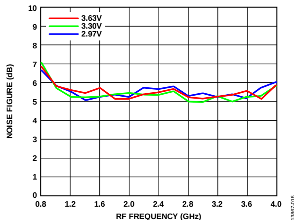
Figure 18. Noise Figure vs. RF Frequency at Various V_{CCQ} , 56 MHz Filter
