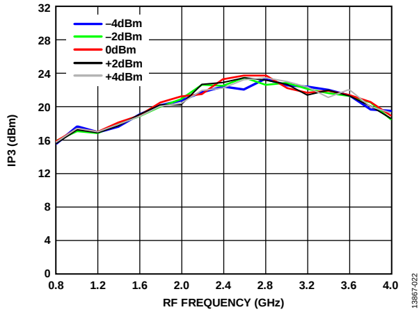
Figure 22. Output IP3 vs. RF Frequency at Various LO Powers, 56 MHz Filter
