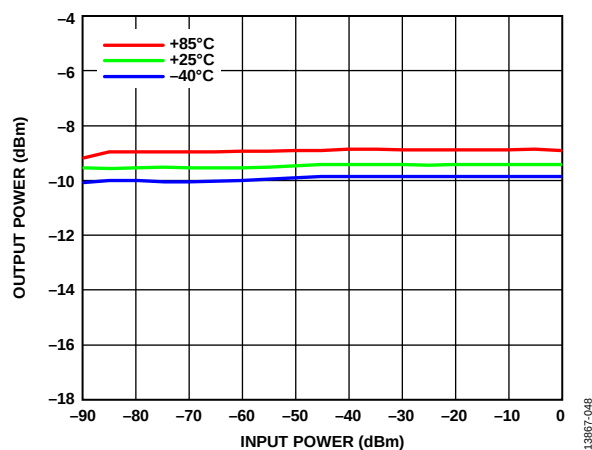
Figure 48. Output Power vs. Input Power over Temperature, RF = 2 GHz
