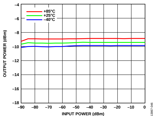
Figure 46. Output Power vs. Input Power over Temperature, RF = 1 GHz
