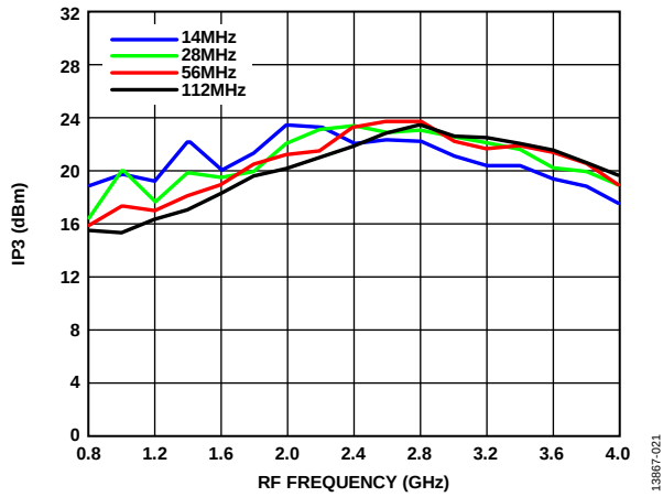
Figure 21. Output IP3 vs. RF Frequency over Internal Filters
