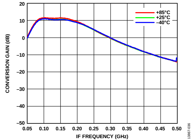
Figure 36. 112 MHz Internal Filter Response vs. IF Frequency at RF = 1 GHz
