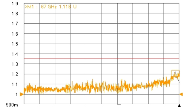
Tr2 S21 Trans LogM RefLvl: 0 dB Res: 1 dB/Div
