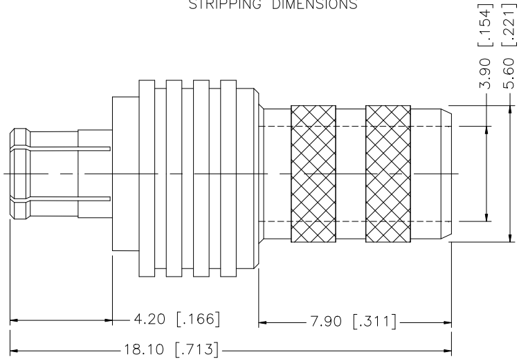
RECOMMENDED CABLE STRIPPING DIMENSIONS
