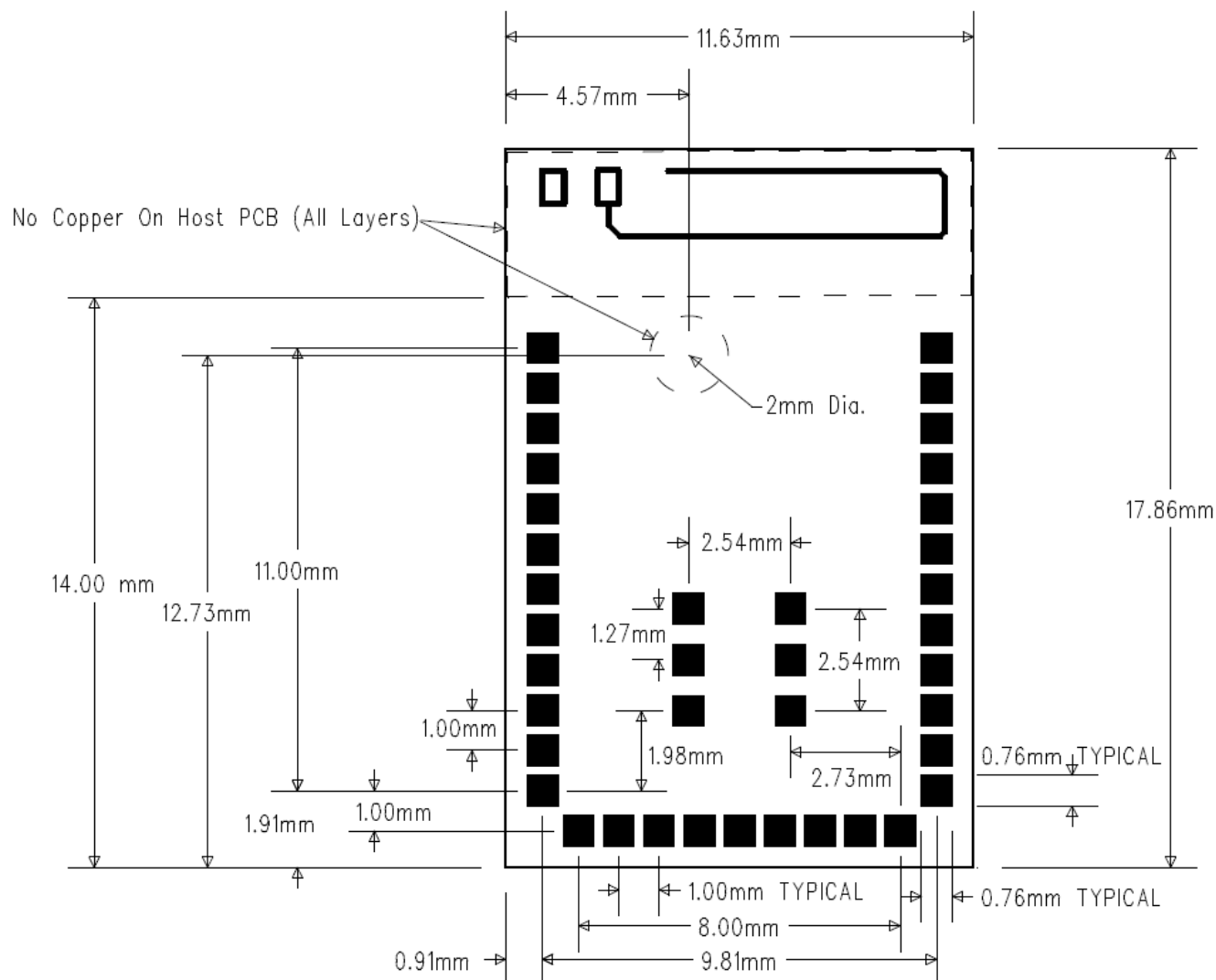
Figure 5 SaBLE-x Recommended PCB Footprint (Viewed from Top)
