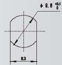
Mounting hole
