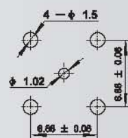
Mounting hole
