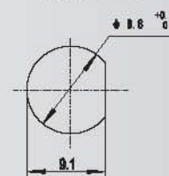
Mounting hole
