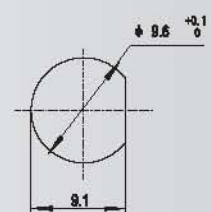
Mounting hole
