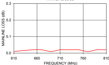
SYBD-28-82HP+ MAINLINE LOSS
