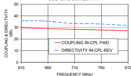
SYBD-28-82HP+ COUPLING & DIRECTIVITY
