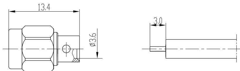
剥线尺寸 stripping dimension
