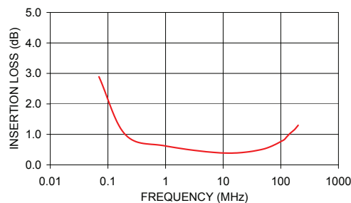
TMO-2-1T+ INSERTION LOSS
