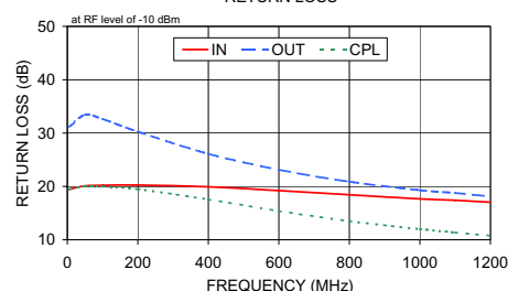
ZX30-9-4+ RETURN LOSS
