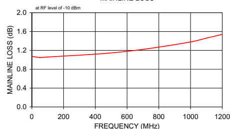
ZX30-9-4+ MAINLINE LOSS
