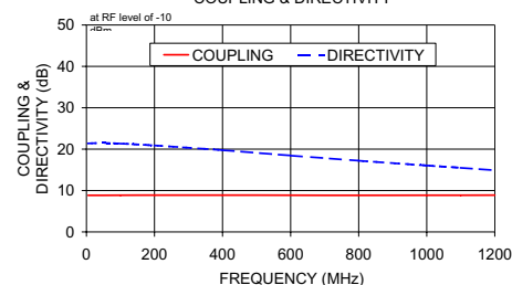
ZX30-9-4+ COUPLING & DIRECTIVITY
