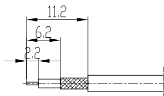
剥线尺寸 stripping dimension
