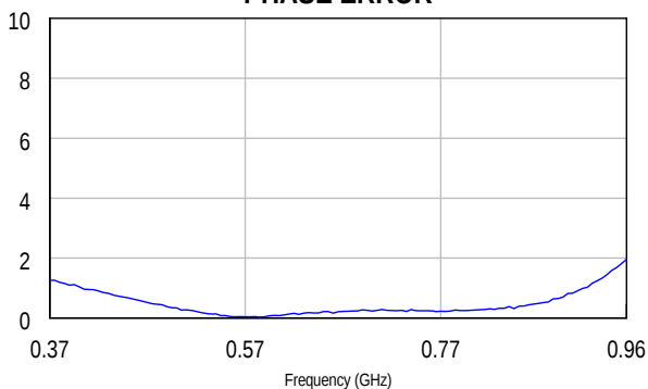
PHASE ERROR
