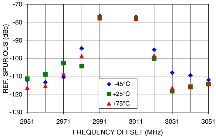
REFERENCE & COMPARISON SPURIOUS Vs FREQ. OFFSET @ Fcar = 3001MHz
