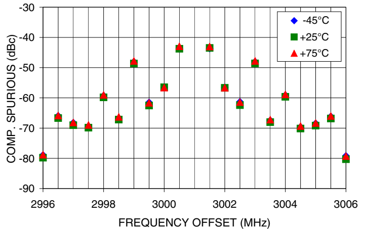
0.5 STEP SIZE & STEP SIZE SPURIOUS Vs FREQ. OFFSET @ Fcar = 3001MHz
