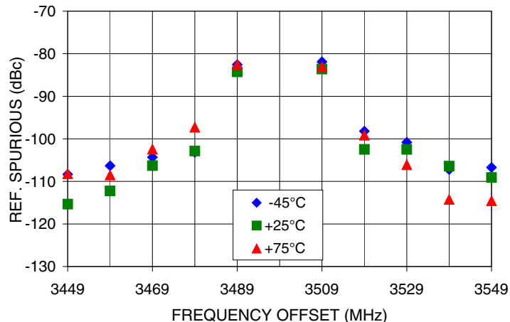
REFERENCE & COMPARISON SPURIOUS Vs FREQ. OFFSET @ Fcar = 3499MHz
