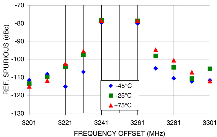
REFERENCE & COMPARISON SPURIOUS Vs FREQ. OFFSET @ Fcar = 3251MHz
