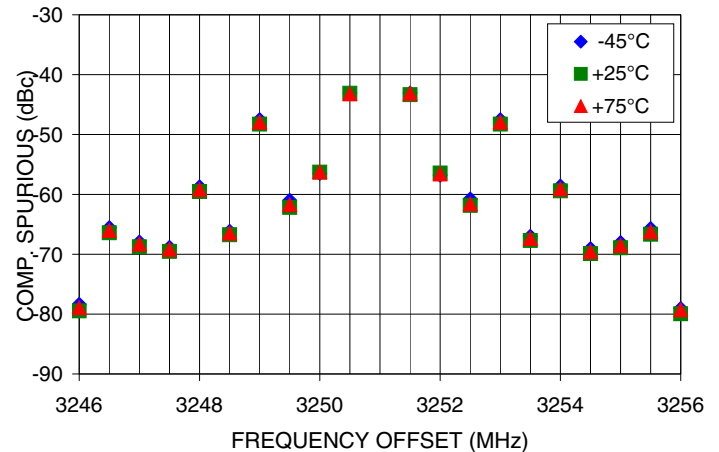
0.5 STEP SIZE & STEP SIZE SPURIOUS Vs FREQ. OFFSET @ Fcar = 3251MHz
