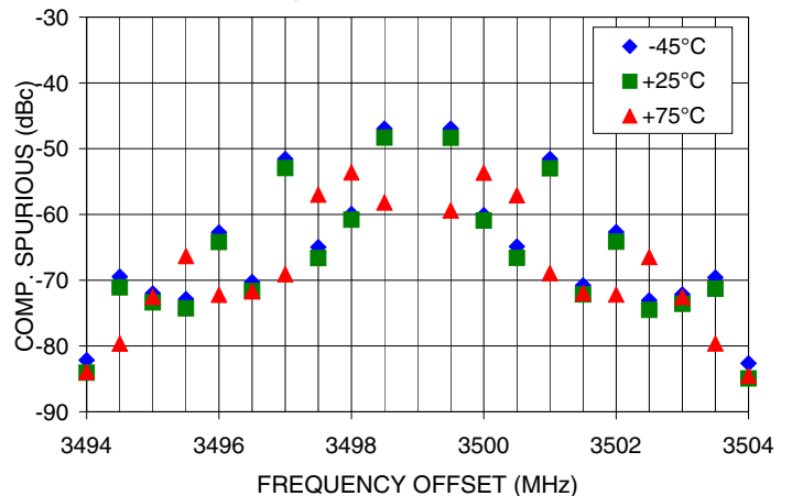
0.5 STEP SIZE & STEP SIZE SPURIOUS Vs FREQ. OFFSET @ Fcar = 3499MHz
