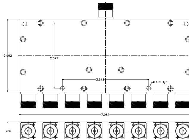
(800-2500 MHz 8-Way Power Divider) (N)
