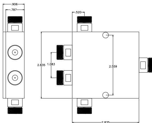
(800-2500 MHz 4-Way Power Divider) (N Connector)
