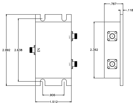
(800-2500 MHz 2-Way Power Divider) (SMA)
