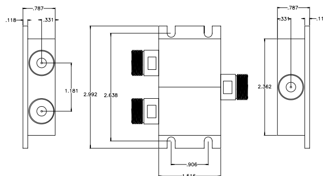
(800-2500 MHz 2-Way Power Divider) (N)
