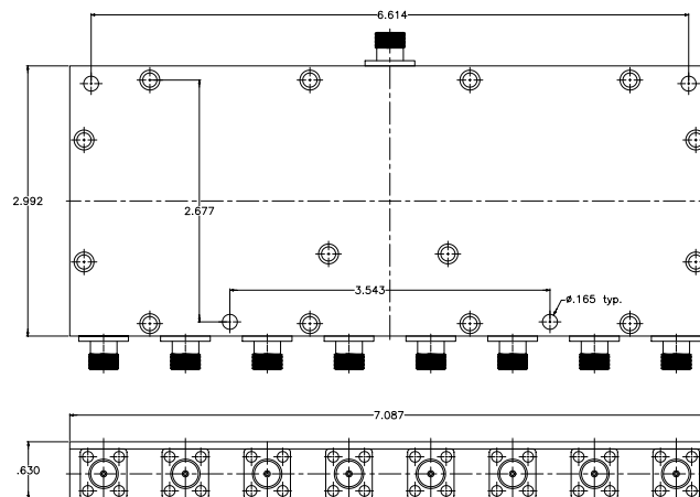
(800-2500 MHz 8-Way Power Divider) (SMA)
