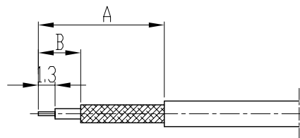
剥线尺寸 stripping dimensions
