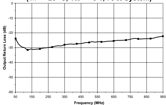
Figure 7: Output Return Loss vs. Frequency ( T_A = +25^\circ\text{C} , V_{DD} = +5\text{ V} , 75\ \Omega System)
