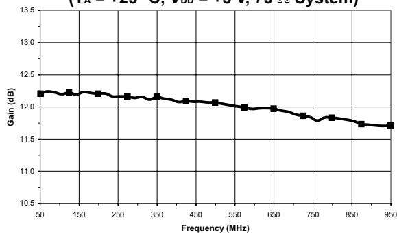
Figure 4: Gain vs. Frequency ( T_A = +25^\circ\text{C} , V_{DD} = +5\text{ V} , 75\ \Omega System)
