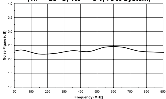
Figure 5: Noise Figure vs. Frequency ( T_A = +25^\circ\text{C} , V_{DD} = +5\text{ V} , 75\ \Omega System)
