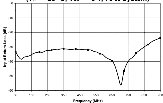
Figure 6: Input Return Loss vs. Frequency ( T_A = +25^\circ\text{C} , V_{DD} = +5\text{ V} , 75\ \Omega System)
