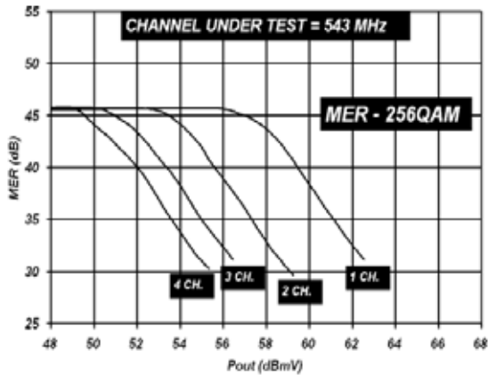
Figure 16: ADA1200 MER – 256 QAM @ 543 MHz
