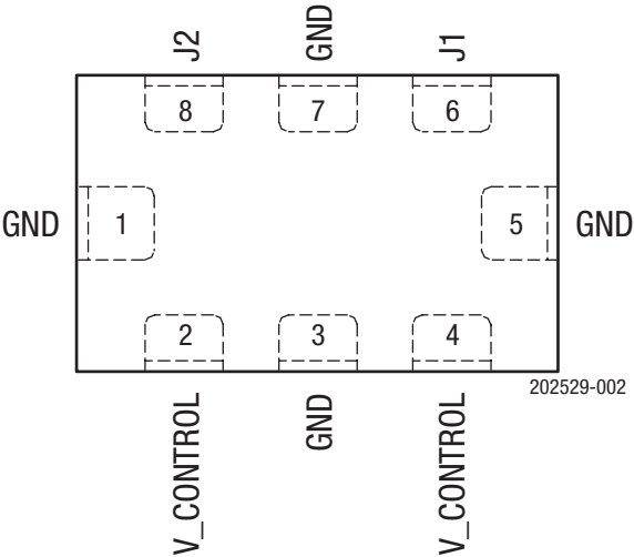
Figure 2. SKY12236-11 Pinout (Top View)
