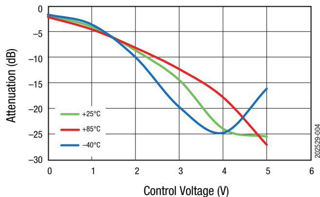
Figure 4. Attenuation vs Control Voltage Over Temperature ( f = 3.8\text{ GHz} )
