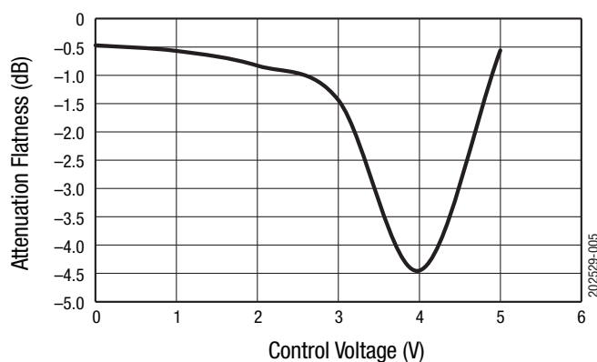
Figure 5. Attenuation Flatness vs Control Voltage ( f = 3.3 to 4.3\text{ GHz} )
