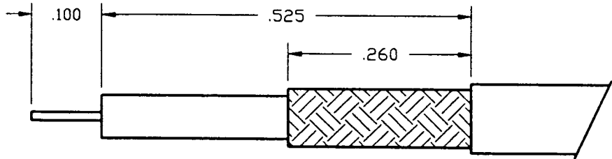
CABLE STRIPPING DIMENSIONS
