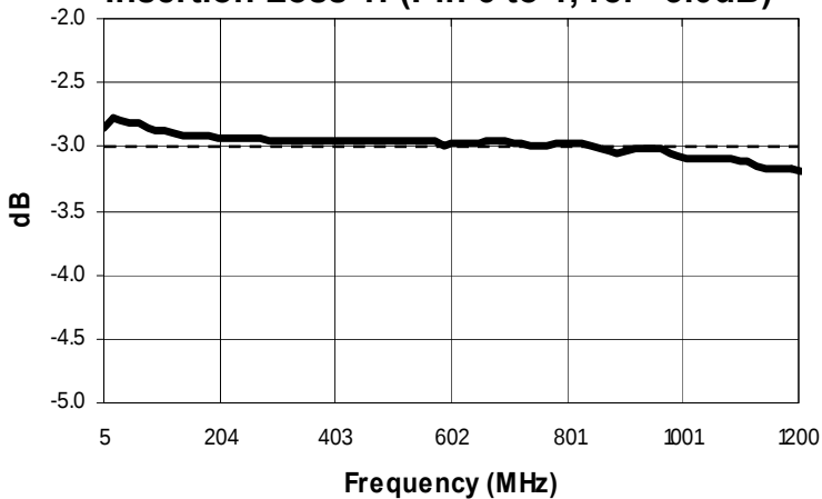
Insertion Loss 1: (Pin 6 to 1, ref -3.0\text{dB} )
