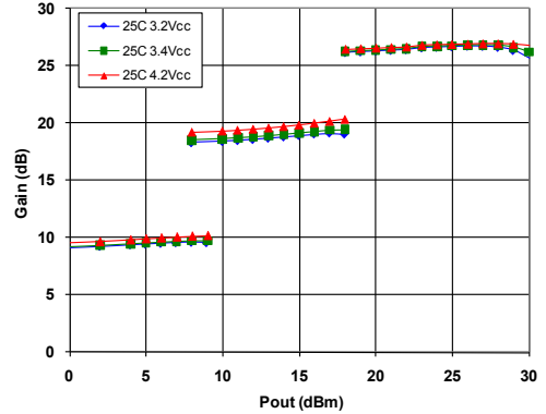
Figure 5: WCDMA Gain (dB) over Voltage ( T_c = 25 °C)
