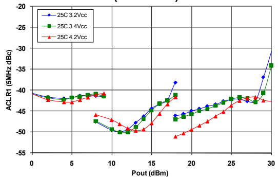
Figure 9: WCDMA ACLR (dBc) over Voltage ( T_c = 25 °C)
