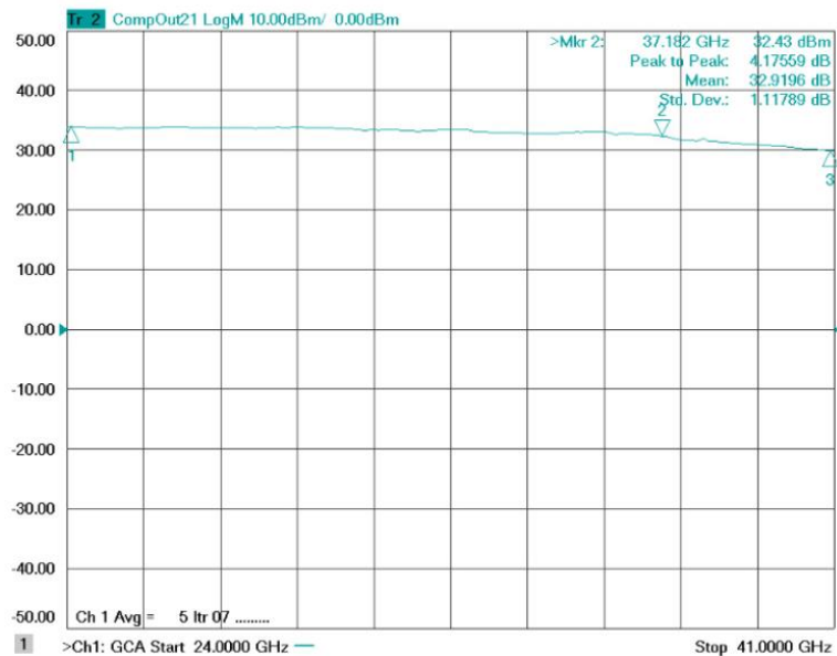
Figure 1-1: ERZ-HPA-2400-4100-33 Psat
