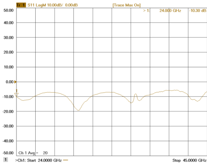
Figure 1-4: ERZ-HPA-2400-4100-33 Input Matching
