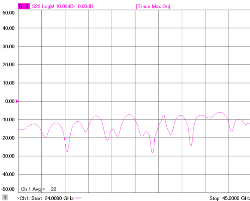
Figure 1-5: ERZ-HPA-2400-4100-33 Output Matching
