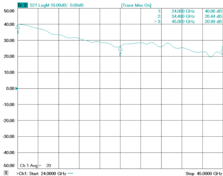
Figure 1-2: ERZ-HPA-2400-4100-33 Small Signal Gain
