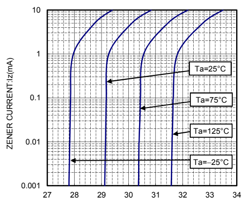
ZENER VOLTAGE: V_z (V) V_z - I_z CHARACTERISTICS
