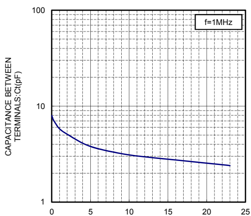
REVERSE VOLTAGE: V_R (V) V_R - C_j CHARACTERISTICS
