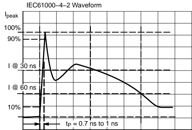
Figure 8. IEC61000-4-2 Spec
