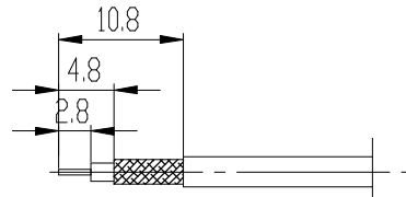
剥线尺寸 stripping dimension
