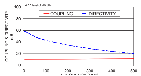
ZFDC-10-1+ COUPLING & DIRECTIVITY
