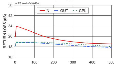
ZFDC-10-1+ RETURN LOSS
