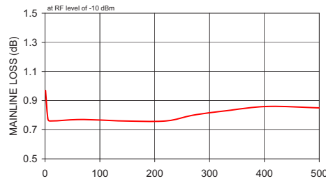
ZFDC-10-1+ MAINLINE LOSS
