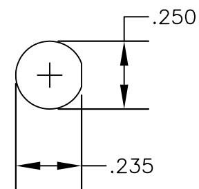
MOUNTING HOLE
