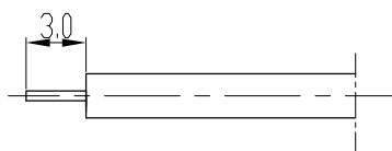
剥线尺寸 stripping dimensions
