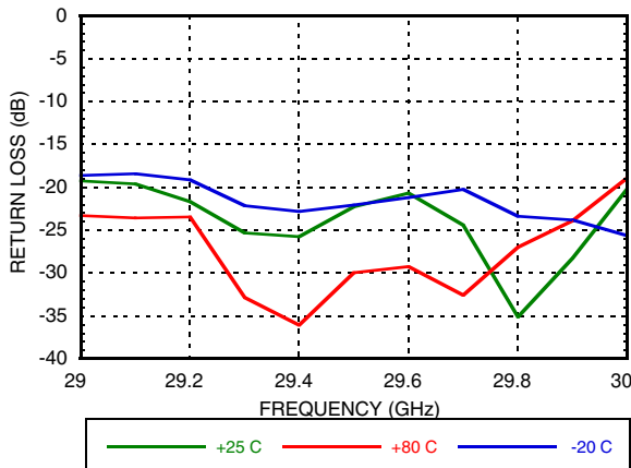
Figure 8. Output Return Losses (Commercial Band)
