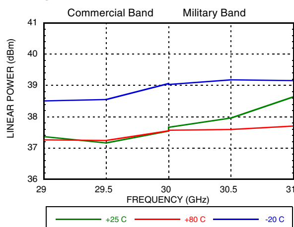
Figure 4. Linear Power (SRG)
