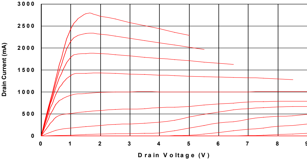
Example of DC I-V Curves Vg = 0.0 V to -2.75 V in 0.25 steps TA = 25°C
