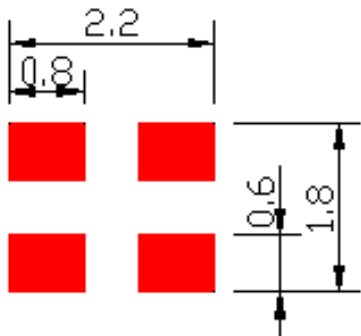
Typical PCB Footprint
