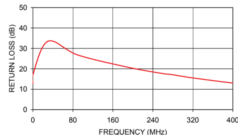
ADT3-6T INPUT RETURN LOSS
