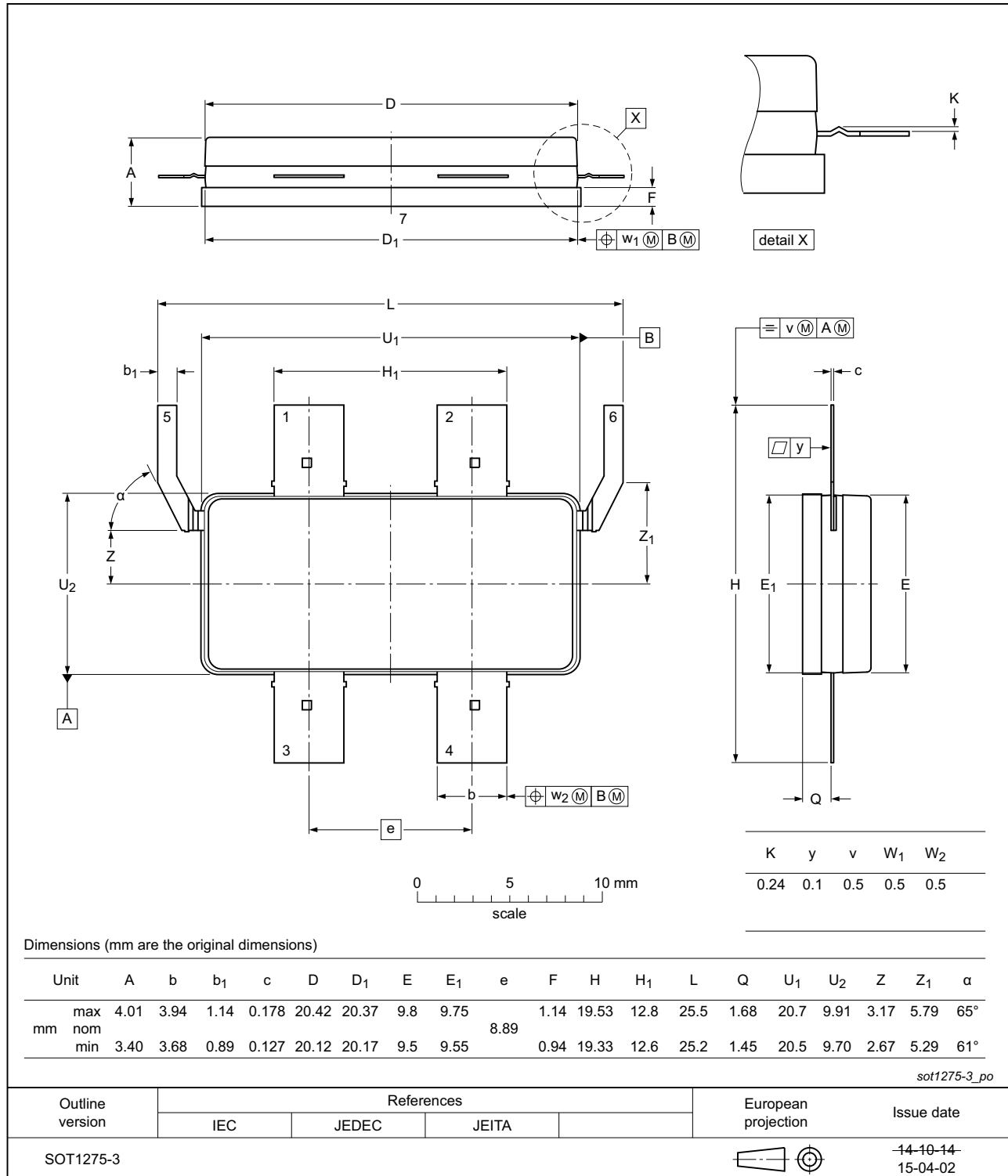
Fig 14. Package outline SOT1275-3
