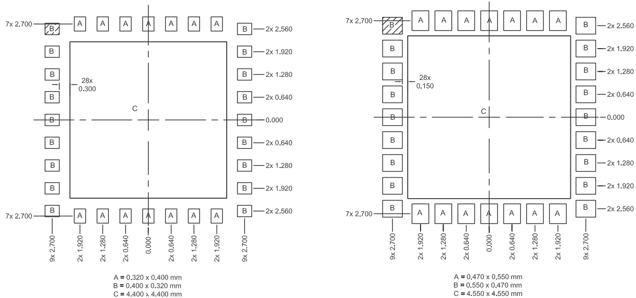
PCB METAL PATTERN
