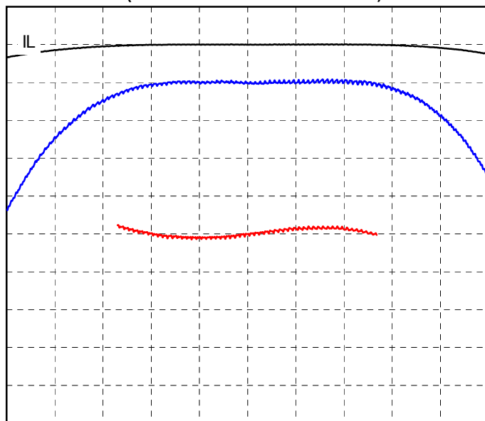
Frequency Response (Best Fit Linear Phase Removed)
