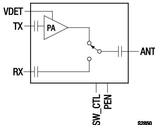
Figure 1. SKY85702-11 Block Diagram
