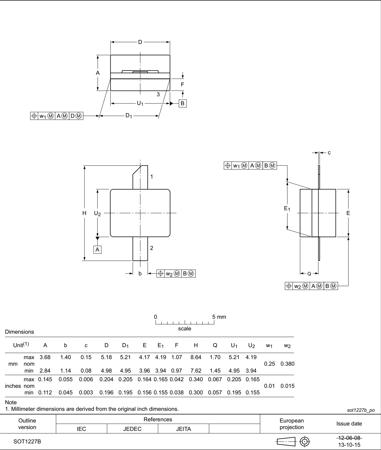
Fig 11. Package outline SOT1227B
