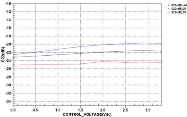
OUTPUT RETURN LOSS VS. CONTROL VOLTAGE VS. TEMPERATURE @ 2350 MHz
