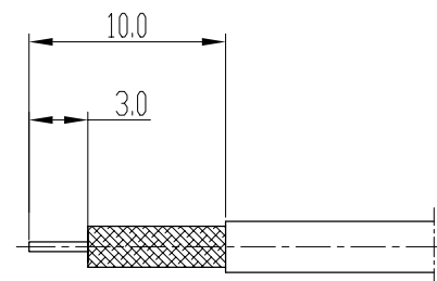
剥线尺寸 stripping dimension
