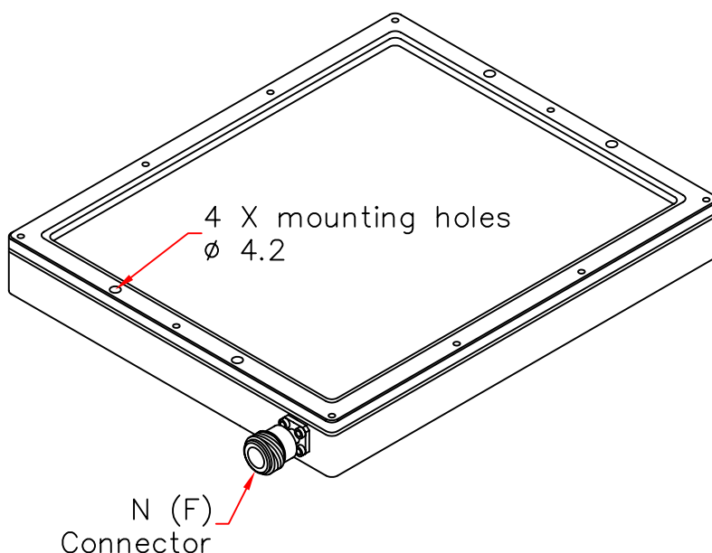
ISOMETRIC VIEW
