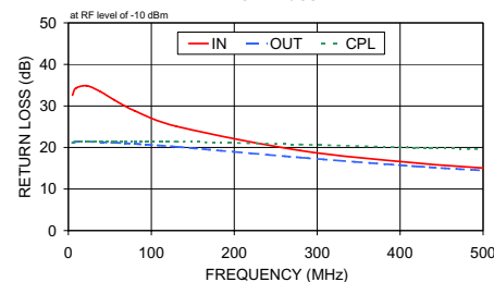
LRDC-10-1J RETURN LOSS
