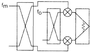
SDM, SML-A...D Single-Sideband Upconverter LO and 1/2 LO
