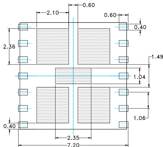
Figure 4: PCB Footprint
