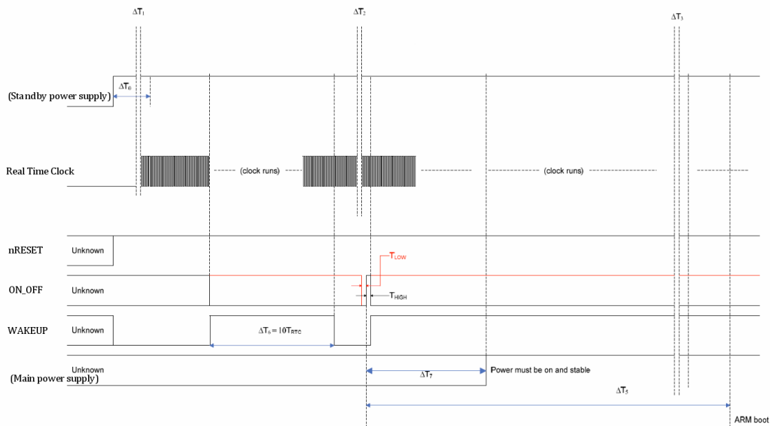
Figure 9-1: Startup timing
