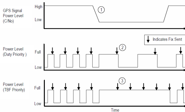
Figure 5-3: APM™ timing
