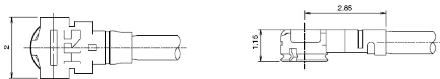
Figure 12-2: ORG1408 receptacle mechanical drawing
