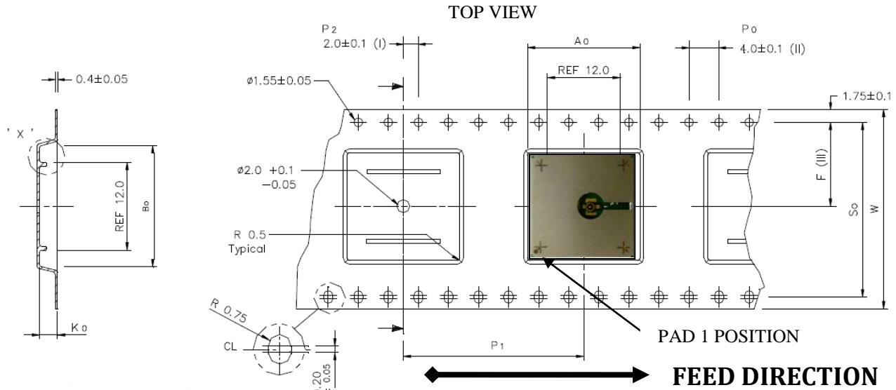
Figure 11-1: Carrier
