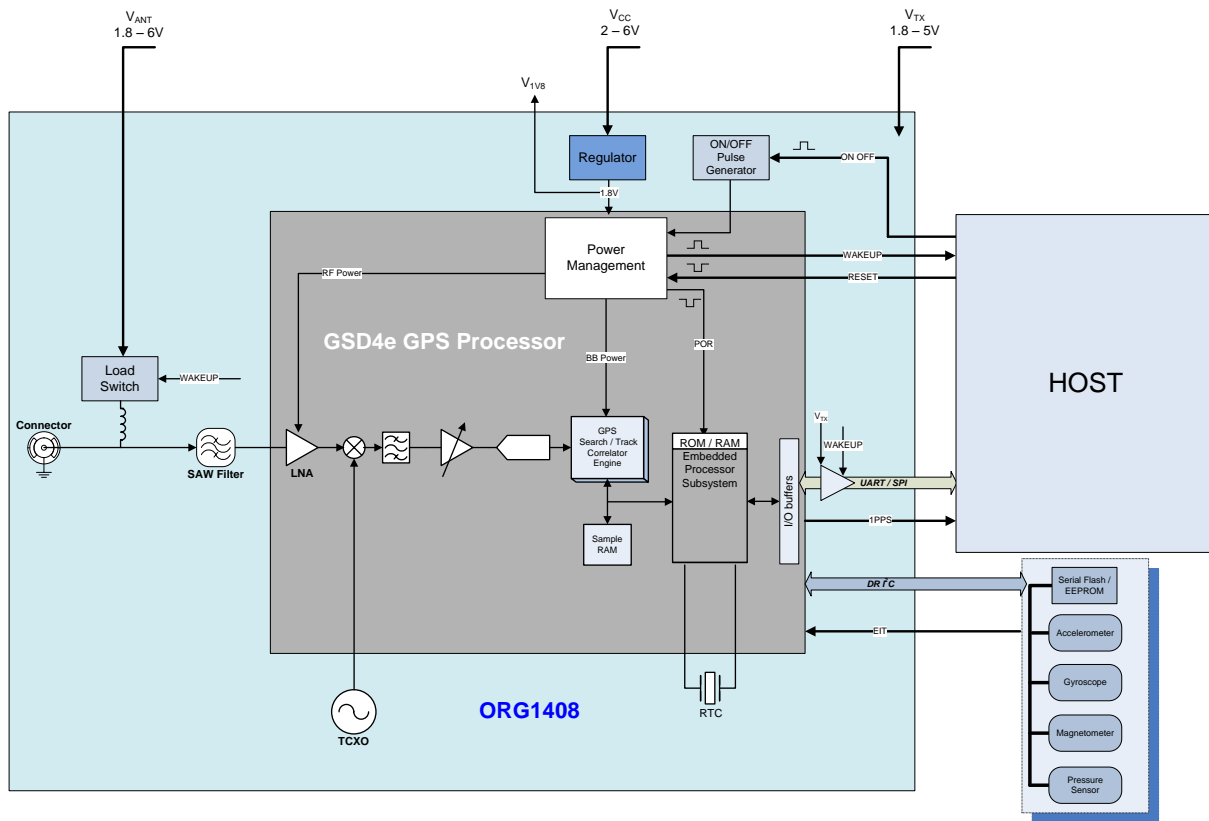
Figure 2-1: ORG1408 architecture
