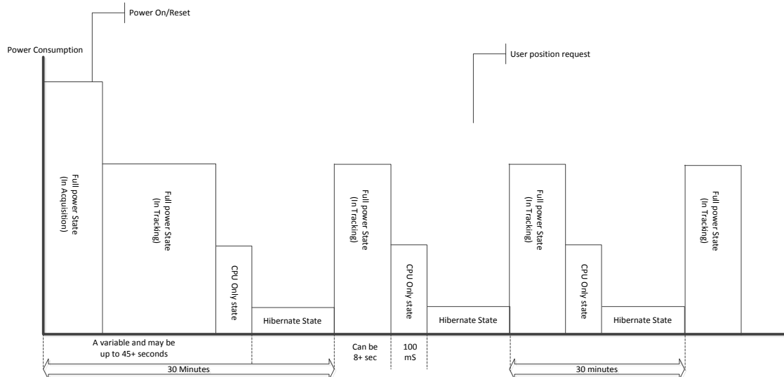
Figure 5-2: PTF™ timing
