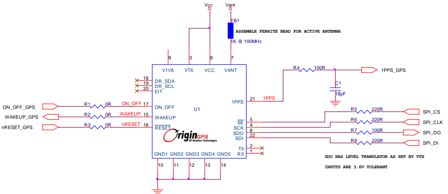
Figure 7-5: SPI interface circuit
