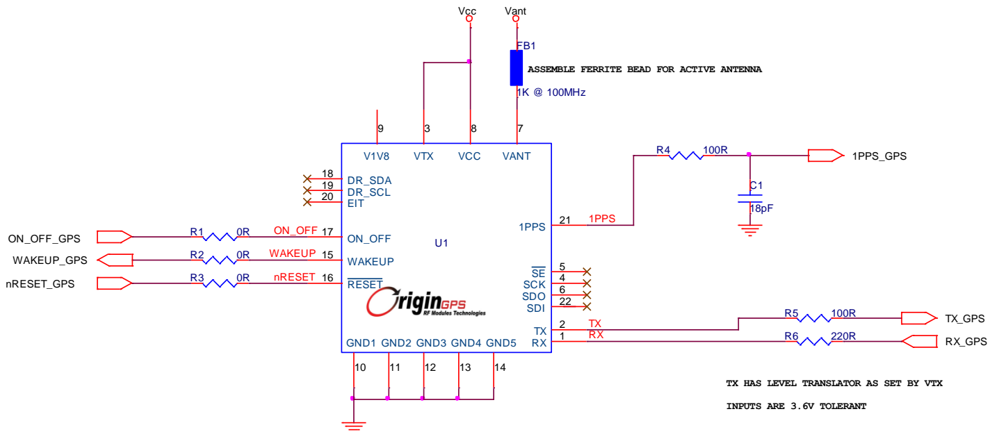
Figure 7-4: UART interface circuit
