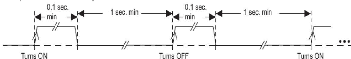
Figure 7-1: ON_OFF timing
