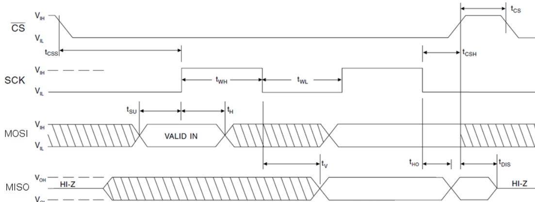
Figure 7-3: SPI timing
