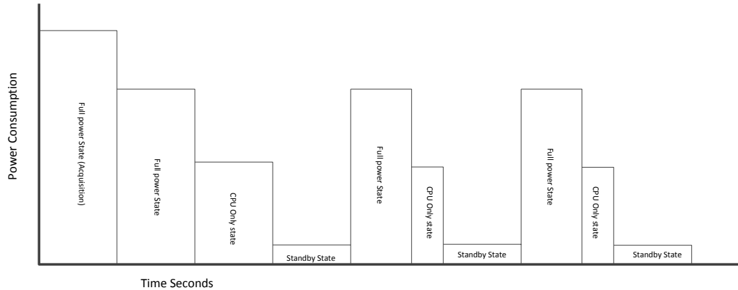
Figure 5-1: ATP™ timing
