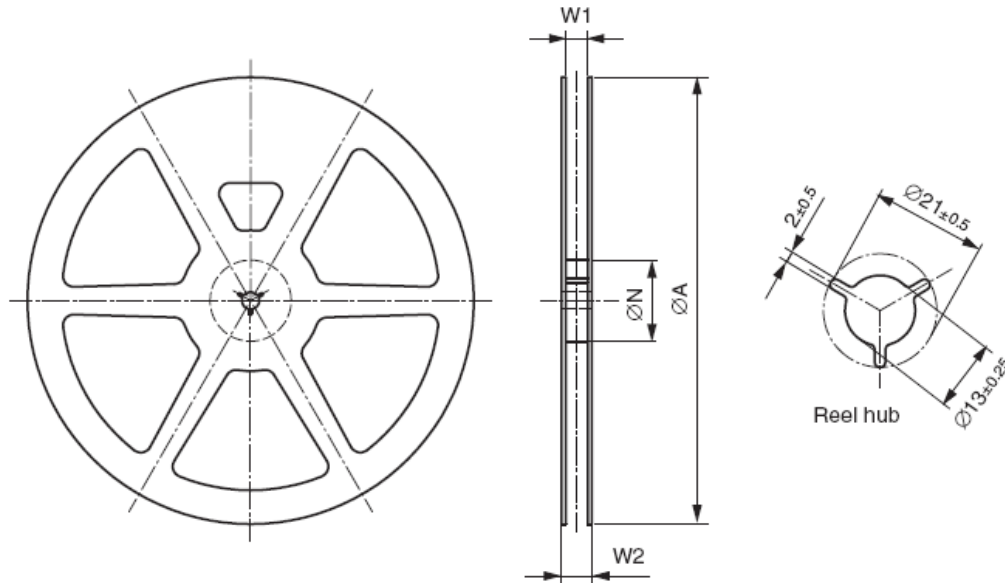
Figure 11-3: Reel
