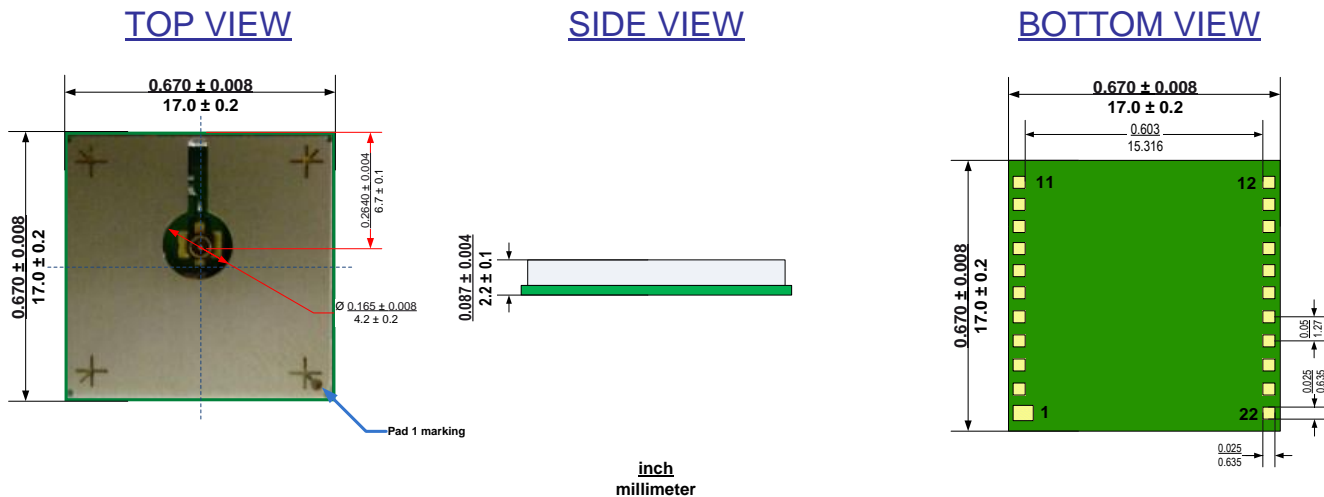
Figure 12-1: ORG1408 mechanical drawing
