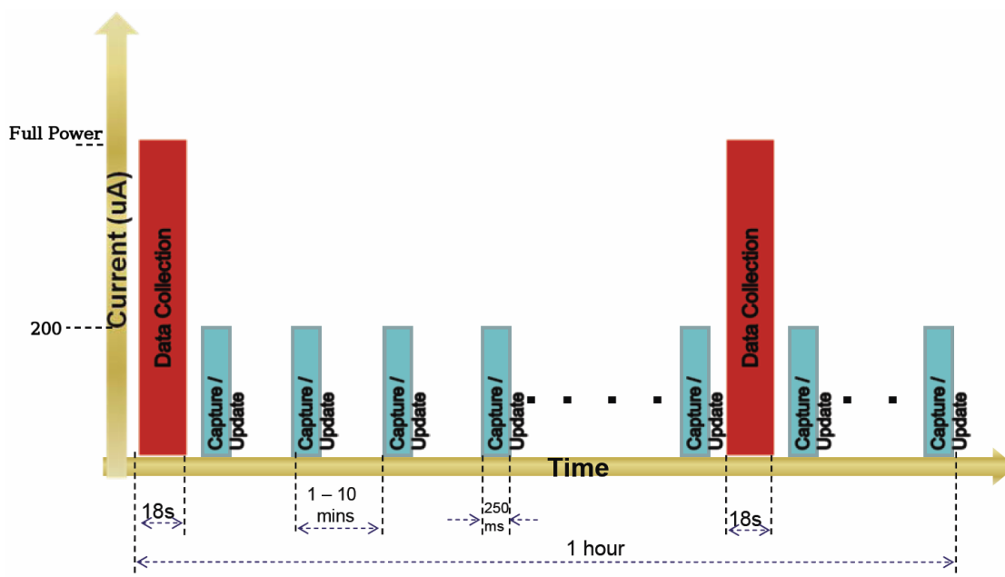
Figure 5-4: MPM™ timing
