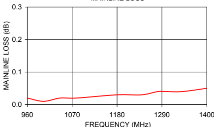
SYBD-24-142HP+ MAINLINE LOSS
