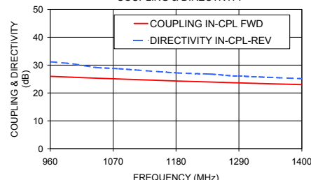
SYBD-24-142HP+ COUPLING & DIRECTIVITY
