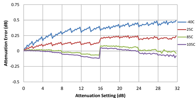
Figure 26. Attenuation Error @ 1800 MHz vs. Temperature
