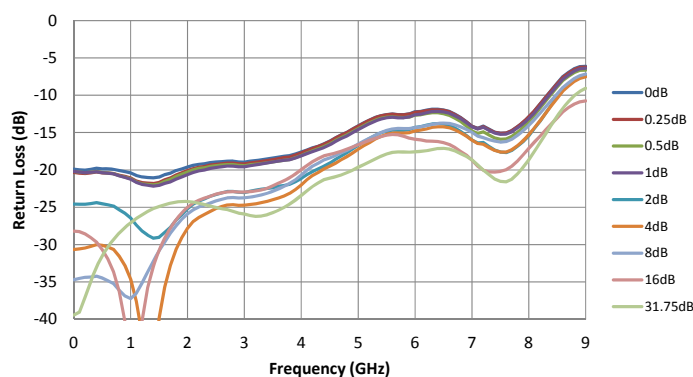
Figure 20. Output Return Loss vs. Attenuation Setting
