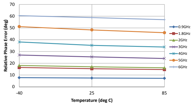
Figure 24. Relative Phase Error for 31.75 dB Attenuation Setting vs. Frequency
