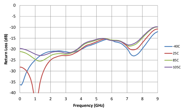
Figure 22. Output Return Loss vs. Temperature for 16 dB Attenuation Setting
