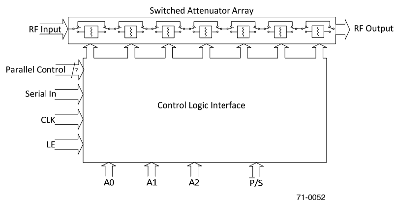
Figure 1. Functional Diagram
