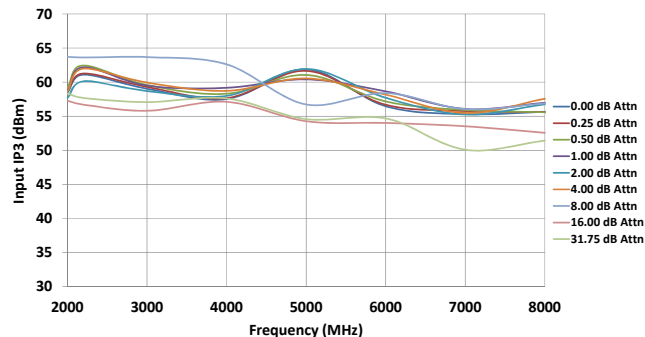
Figure 28. IIP3 vs. Attenuation Setting
