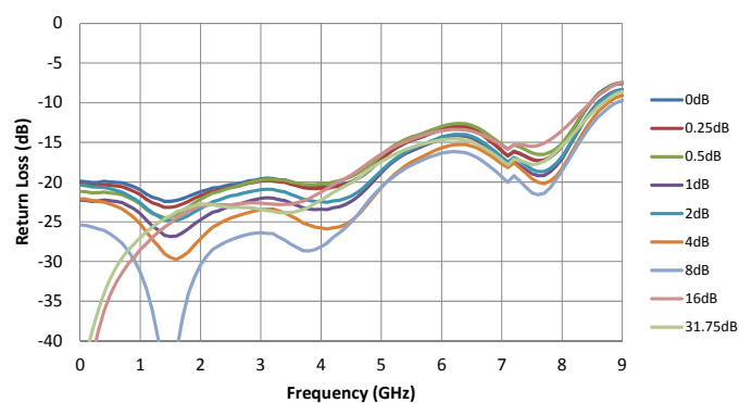
Figure 19. Input Return Loss vs. Attenuation Setting
