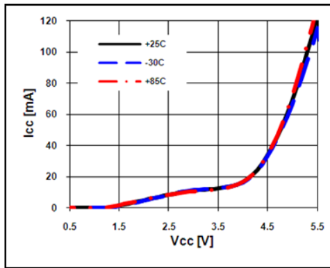
V-I Characteristics
