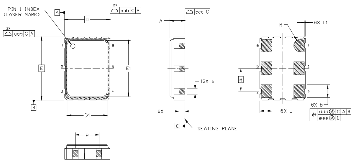
Figure 3. Si515 Outline Diagram
