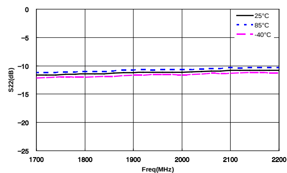
Output Return Loss vs. Frequency
