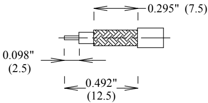
STRIPPING DIMENSION
